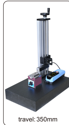
Heavy duty test stand SR200-STD (optional)
