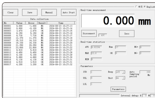
Software
